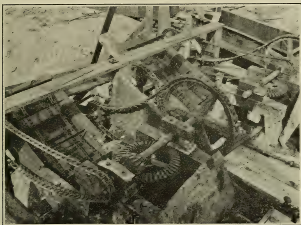
FIG. 27.—Looking into the Top of the Extracting Apparatus.
